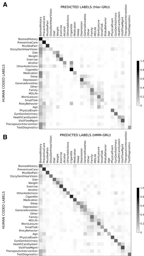
Figure 6. Confusion matrices generated by (A) hierarchical gated recurrent units (Hier-GRU) and (B) hidden Markov model gated recurrent units (HMM-GRU), where the intensity of each cell shows the conditional probabilities of p(\text{predicted label} | \text{human-coded label}) and each row sums to 1. A number of subsets of topics have high confusion probabilities, including Diet/Weight/Exercise, Depression/GeneralAnxieties, and Family/MDLife/WorkLeisure.
