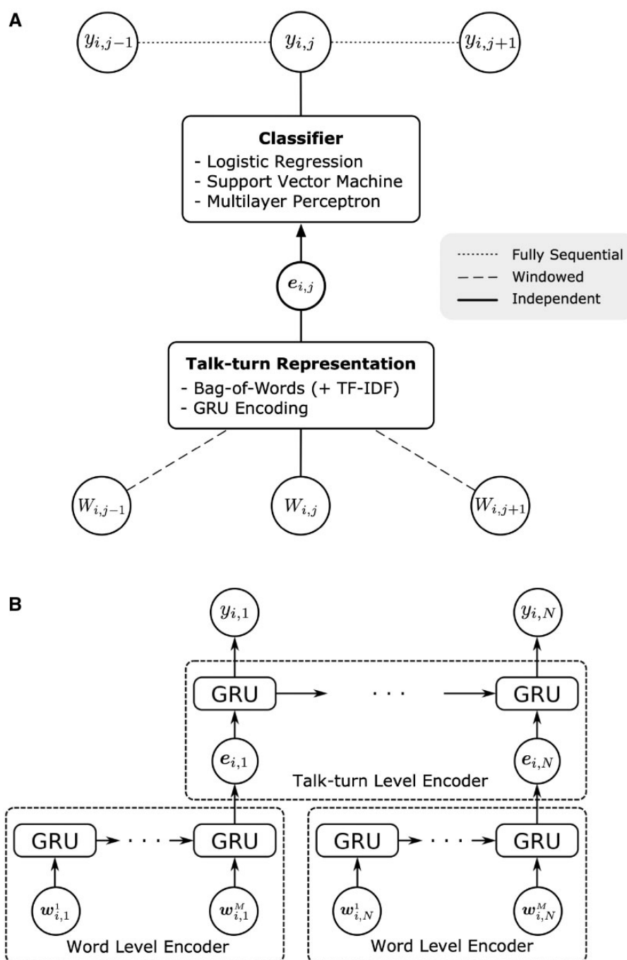
Figure 2. (A) A high-level diagram of the various models discussed in the article. i, j stands for talk-turn j in session i . W_{i,j} is the list of tokenized words in talk-turn j . For each talk-turn j , we first generate the vectorized talk-turn representation e_{i,j} and the talk-turn representation e_{i,j} is used as an input to different classifiers to predict the topic label y_{i,j} , which is the topic label for talk-turn j . Windowed models use the adjacent talk-turns to create the talk-turn-level representation, and the fully sequential models make use of the sequential dependencies between the topic labels. (B) Simplified diagram of the hierarchical gated recurrent units (Hier-GRU). Each one-hot-encoded word vector in talk-turn j in visit i (shown as w_{i,j,k} for the k -th word in talk-turn j ) is fed into the word level encoder to get a talk-turn representation e_{i,j} , which becomes the input to the talk-turn-level encoder. The model has dependencies at the hidden state of talk-turn-level gated recurrent units (GRUs). In our experiments, both encoders were bidirectional.
